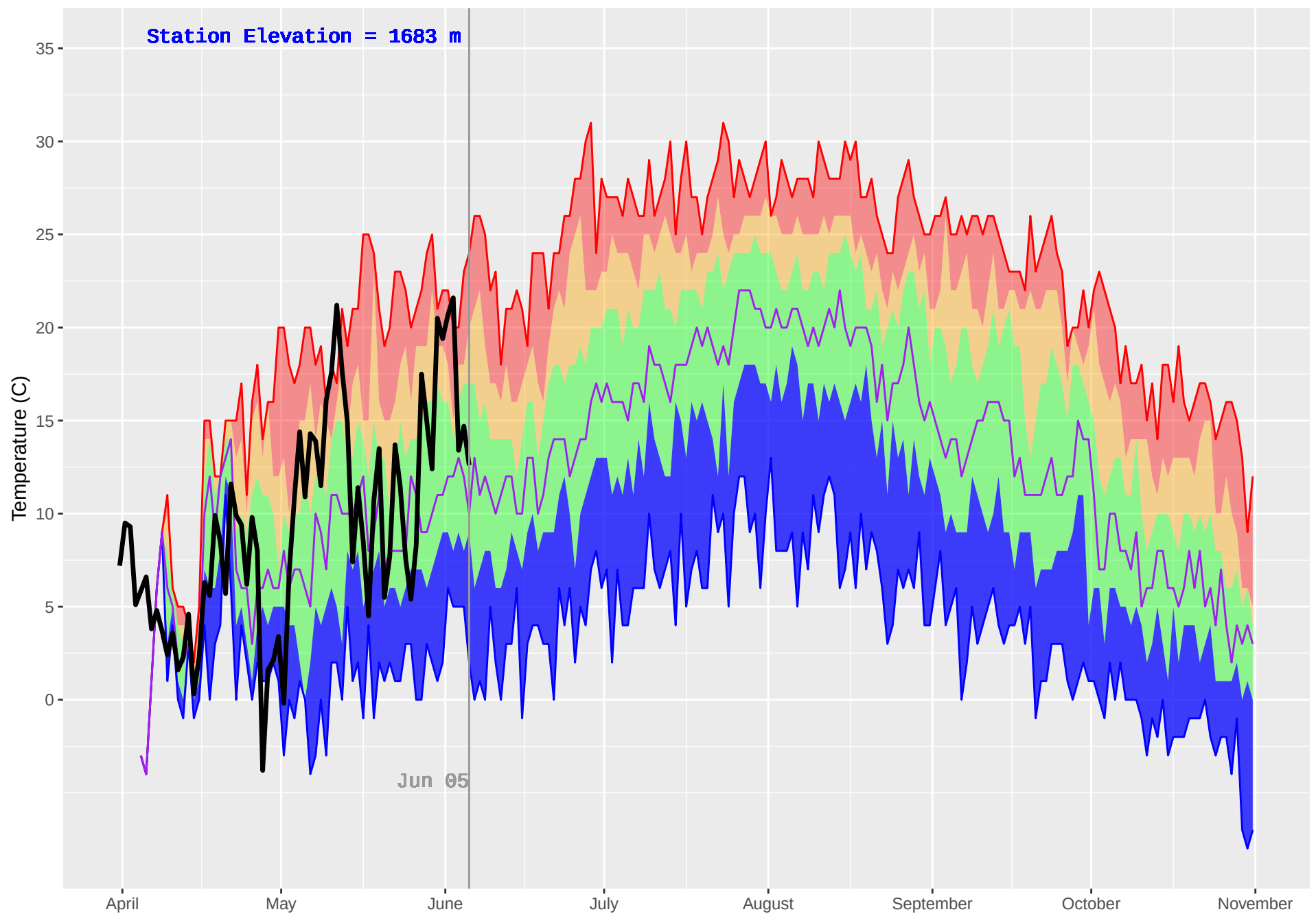
ASHNOLA (331) : Historical (1992–2018) and Current (2019) Daily Temperature
