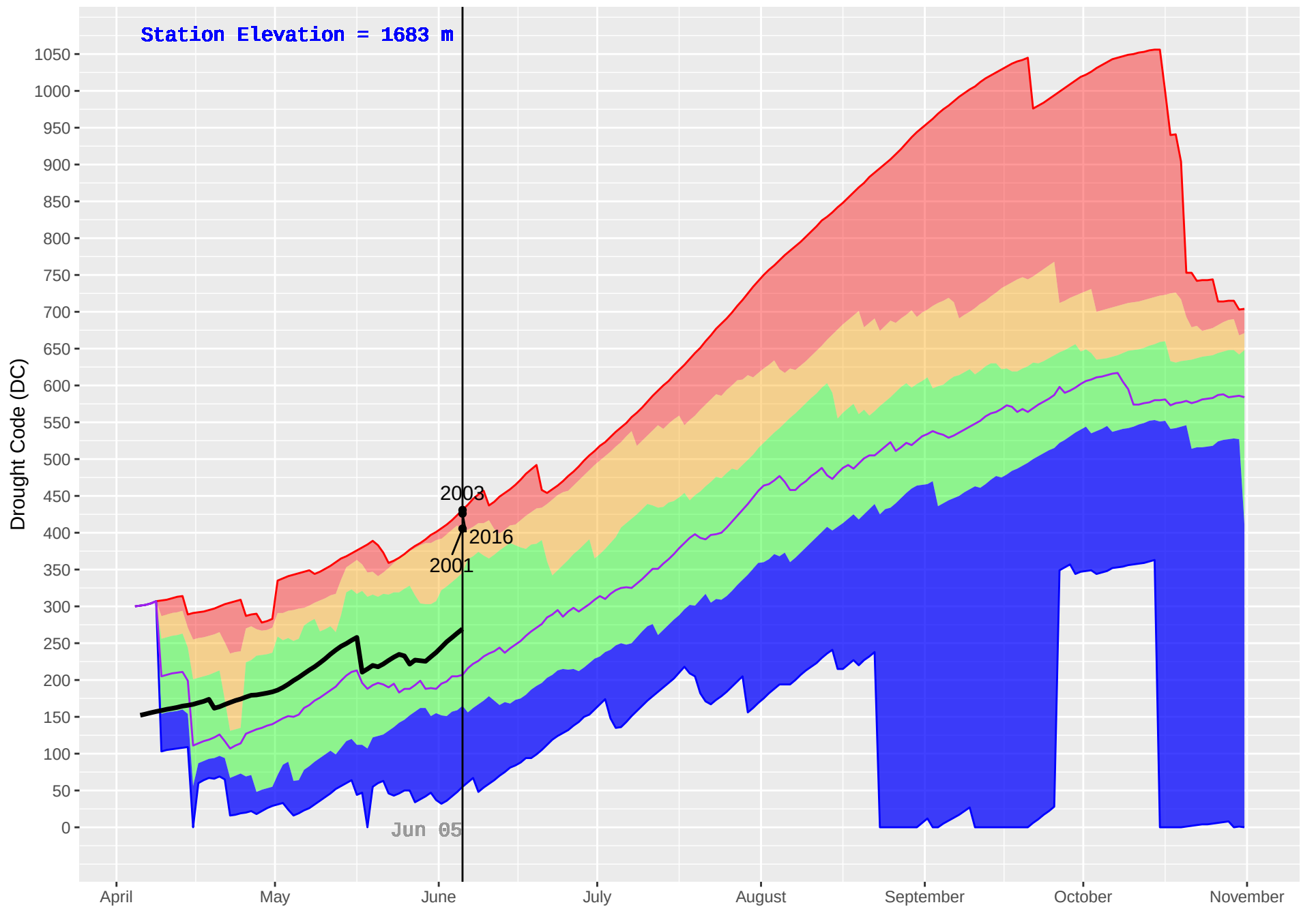
ASHNOLA (331) : Historical (1992–2018) and Current (2019) Daily Drought Code (DC)
