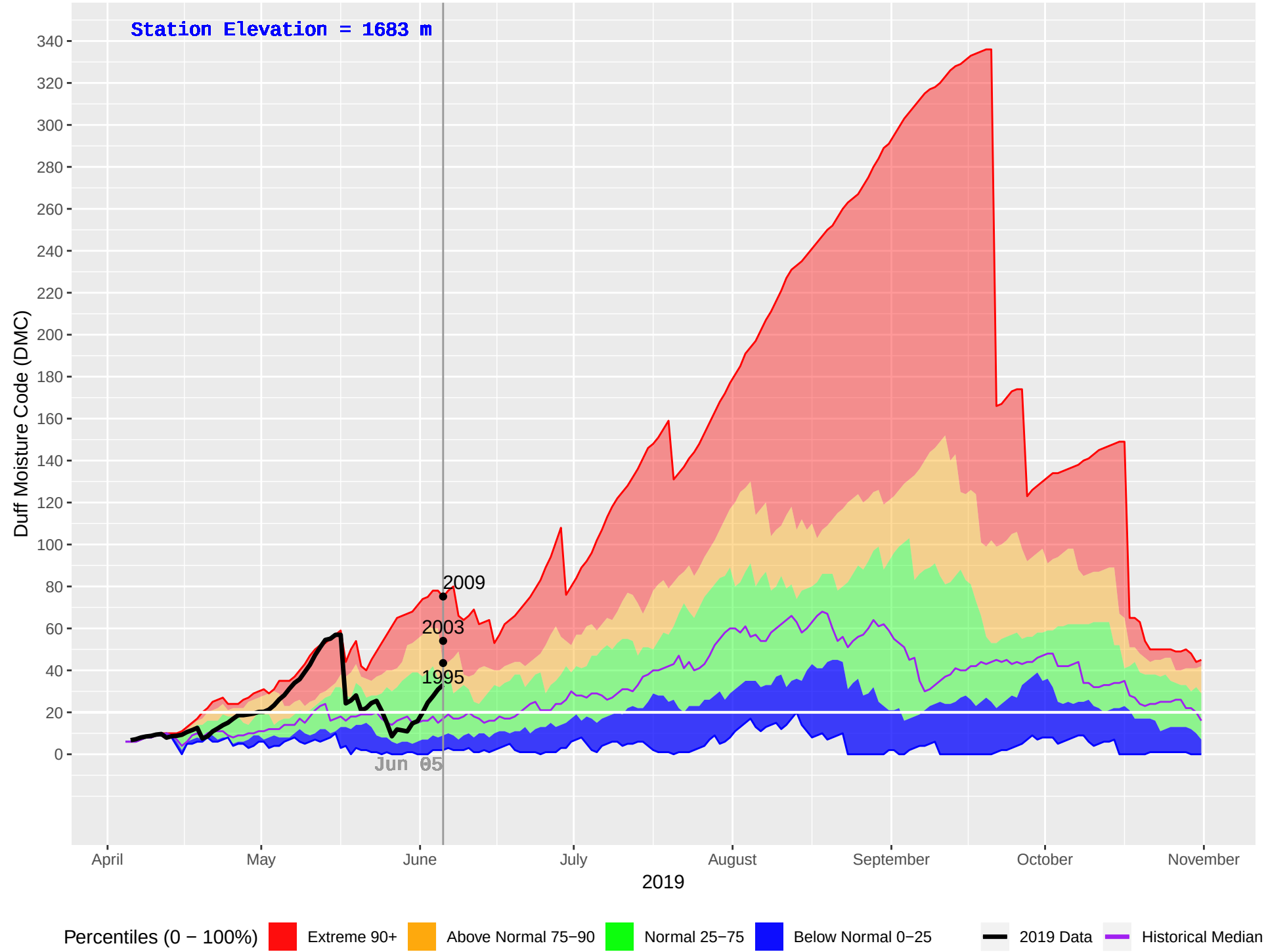
ASHNOLA (331) : Historical (1992–2018), Current (2019) Daily Duff Moisture Code (DMC)
