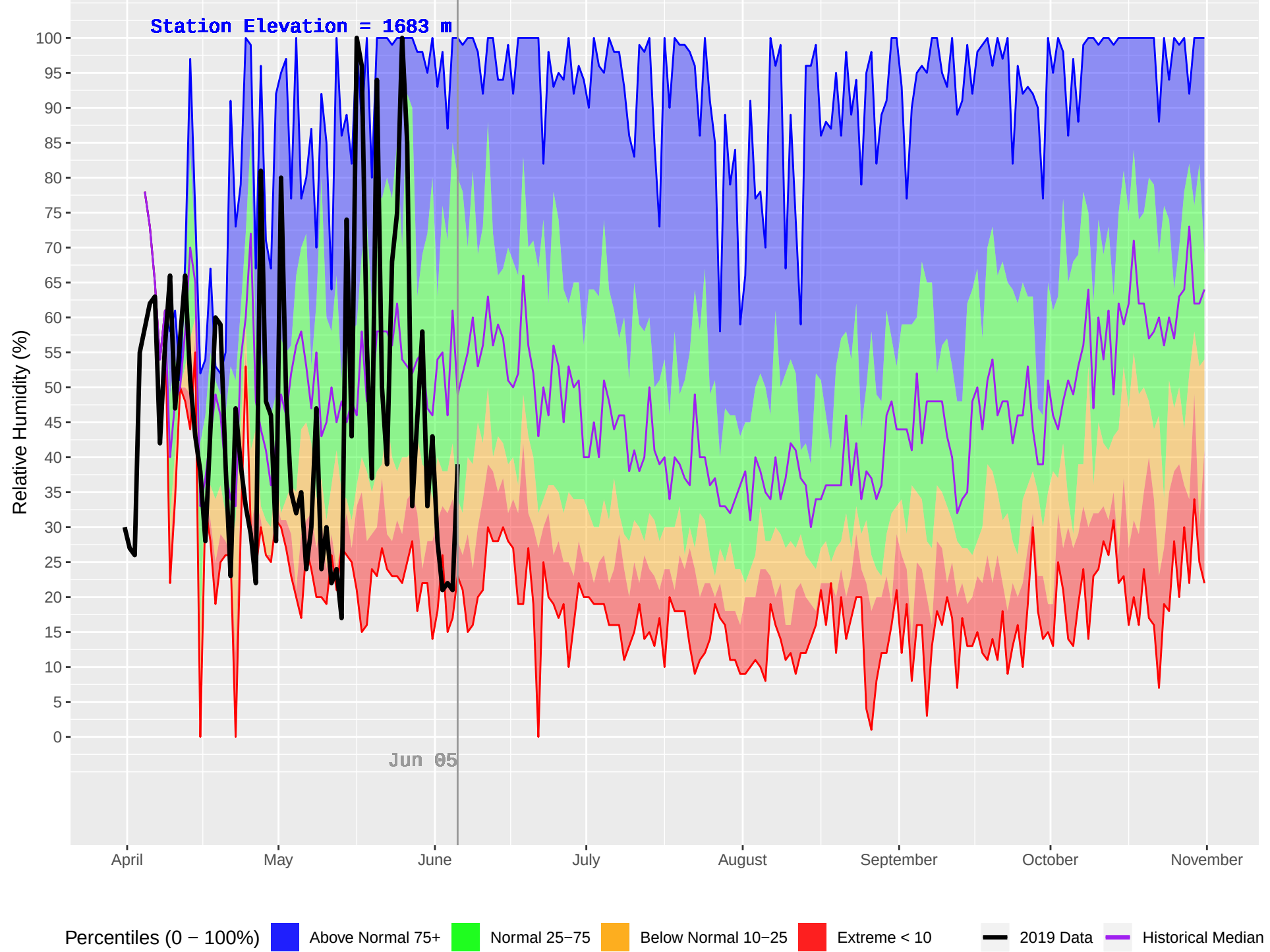
ASHNOLA (331) : Historical (1992–2018) and Current (2019) Daily Relative Humidity
