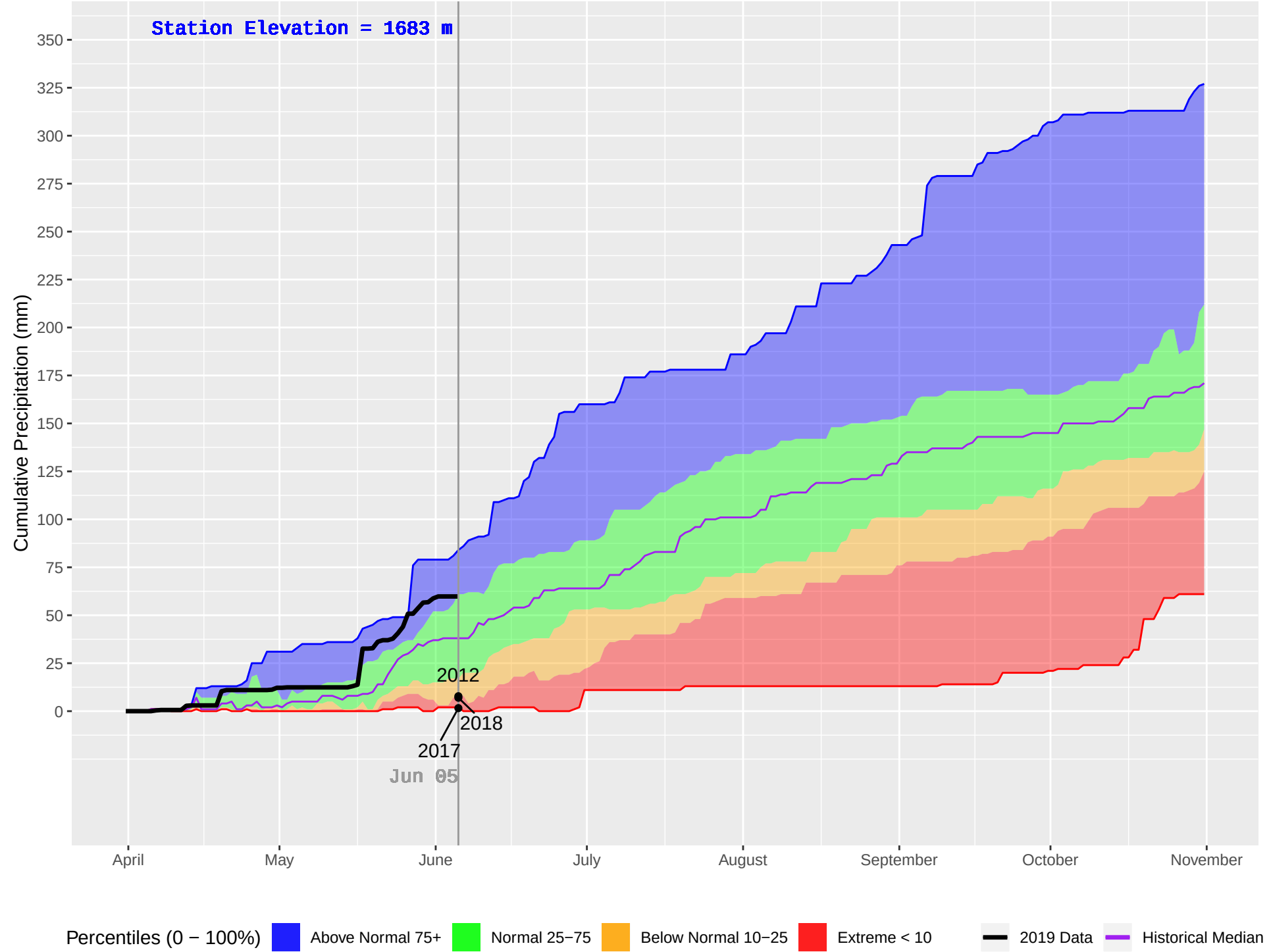
ASHNOLA (331) : Historical (1992–2018), Current (2019) Daily Cumulative Precipitation
