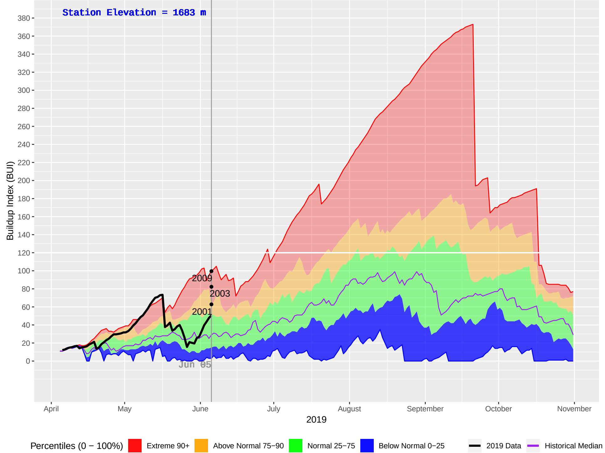
ASHNOLA (331) : Historical (1992–2018), Current (2019) Daily Buildup Index (BUI)
