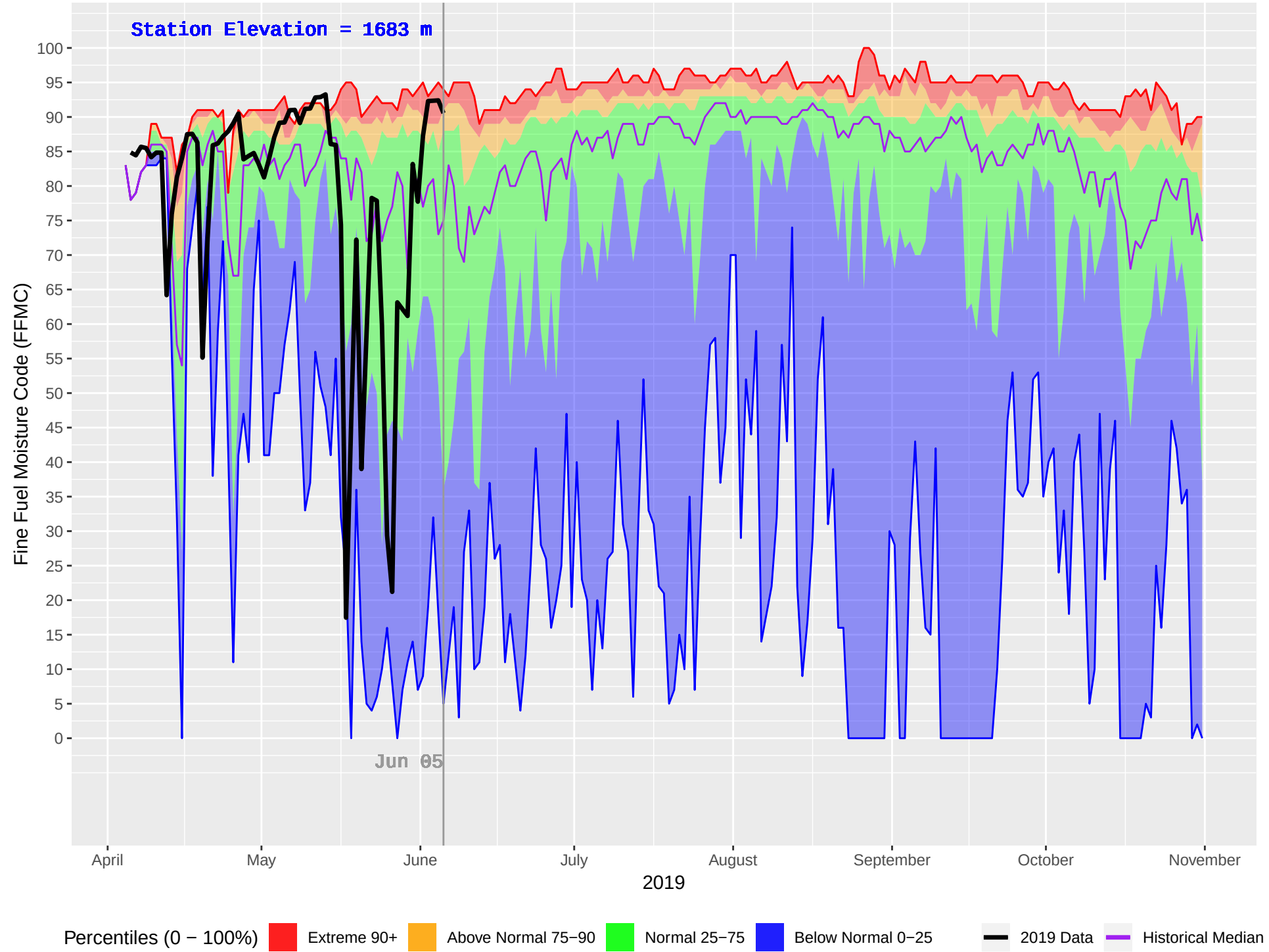
ASHNOLA (331) : Historical (1992–2018) and Current (2019) Daily Fine Fuel Moisture Code (FFMC)
